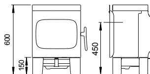
Jøtul F 105 with base and soapstone top
