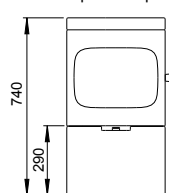
Jøtul F 105 with base and soapstone top
