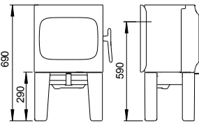
Jøtul F 105 with long legs
