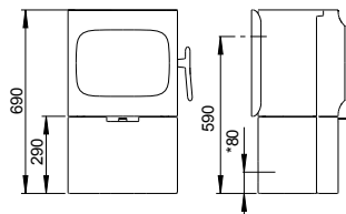
Jøtul F 105 with base
